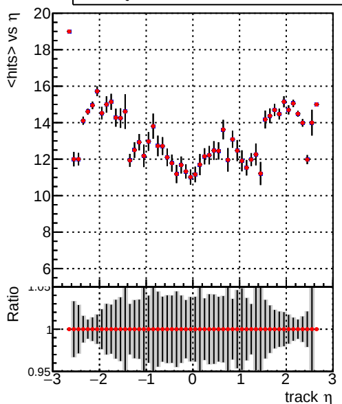
mean hits vs \eta — DQM_V0001_R000000001_Global_mkFit_CANDFINAL100stable — DQM_V0001_R000000001_Global_mkFit_CANDFINAL100stable2
