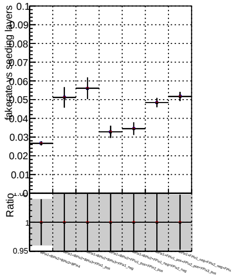
Fake rate vs. — DOM_V0001_R0000000001 Global mkFit CANDEFINAL100stable — DOM_V0001_R0000000001 Global mkFit CANDEFINAL100stable3 — DOM_V0001_R0000000001 Global mkFit CANDEFINAL100stable4444
