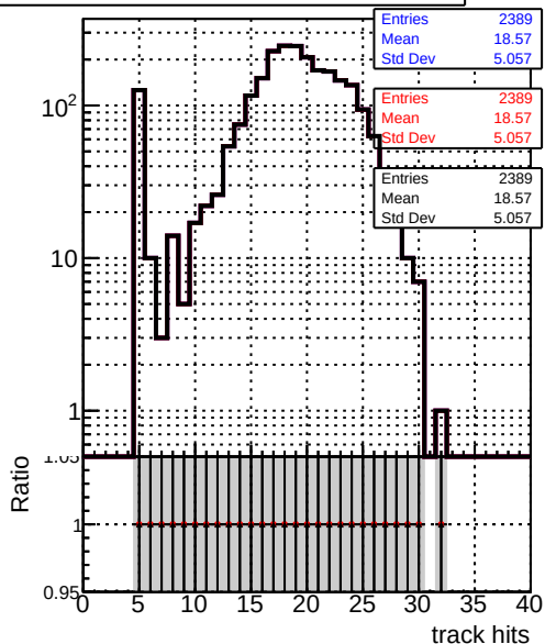
mean hit DQM_V0001_R000000001_Global_mkFit_CANDFINAL100stable DQM_V0001_R000000001_Global_mkFit_CANDFINAL100stable3 DQM_V0001_R000000001_Global_mkFit_CANDFINAL100stable4444
