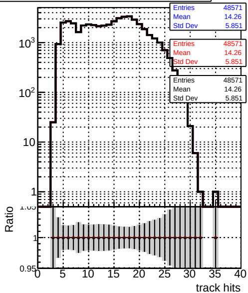
mean hits DQM_V0001_R000000001_Global_mkFit_CANDFINAL100stable DQM_V0001_R000000001_Global_mkFit_CANDFINAL100stable3 DQM_V0001_R000000001_Global_mkFit_CANDFINAL100stable4444
