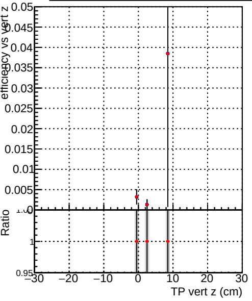
Efficiency vs. TP vert z (cm) Legend: DQM_V0001_R000000001_Global_mkFit_CANDFINAL100stable DQM_V0001_R000000001_Global_mkFit_CANDFINAL100stable3
