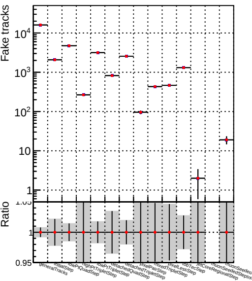
Numbe —●— DQM_V0001_R000000001_Global_mkFit_CANDFINAL100stable3
