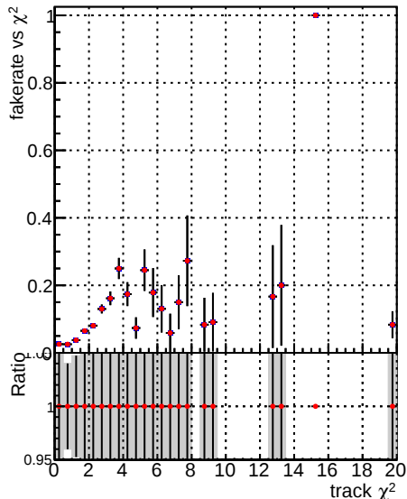
Fake rate vs. Legend Global mkFit CANDFINAL100stable Blue line with dots DQM_V0001_R000000001 Global mkFit CANDFINAL100stable Red line with dots DQM_V0001_R000000001 Global mkFit CANDFINAL100stable3
