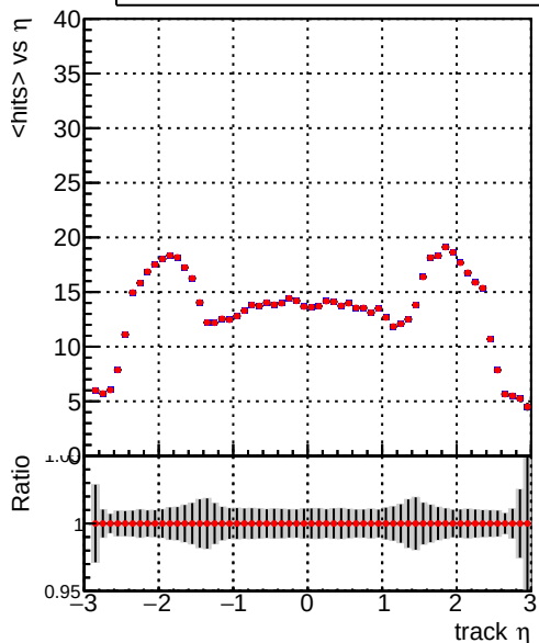
mean hits — DQM_V0001_R000000001_Global_mkFit_CANDFINAL100stable — DQM_V0001_R000000001_Global_mkFit_CANDFINAL100stable3
