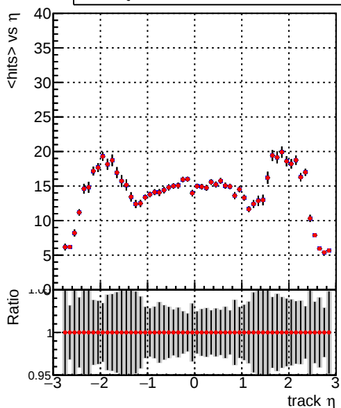
— DQM_V0001_R000000001_Global_mkFit_CANDFINAL100stable — DQM_V0001_R000000001_Global_mkFit_CANDFINAL100stable3
