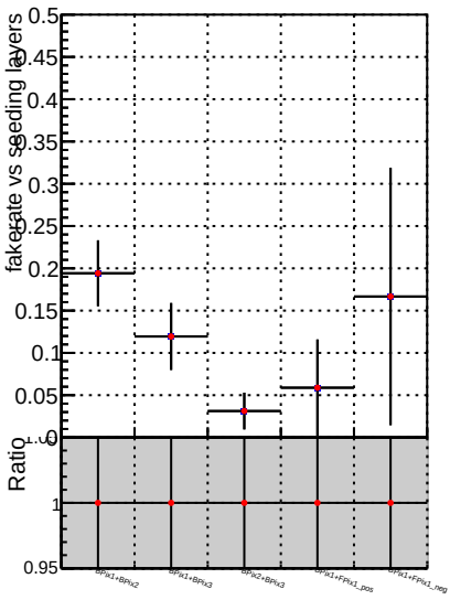
Fake rate vs. — Global mkFit CANDFINAL100stable — Global mkFit CANDFINAL100stable3
