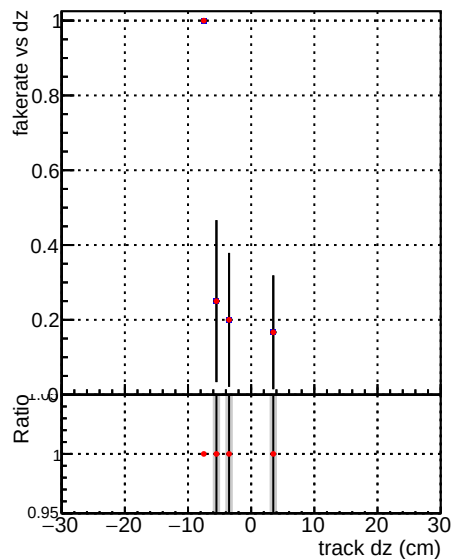
Fake rate vs dz DQM V0001_R000000001 Global mkFit CANDFINAL100stable Fake rate vs dz DQM V0001_R000000001 Global mkFit CANDFINAL100stable3
