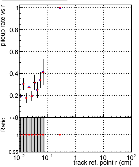
—●— DQM_V0001_R000000001_Global_mkFit_CANDFINAL100stable —●— DQM_V0001_R000000001_Global_mkFit_CANDFINAL100stable3
