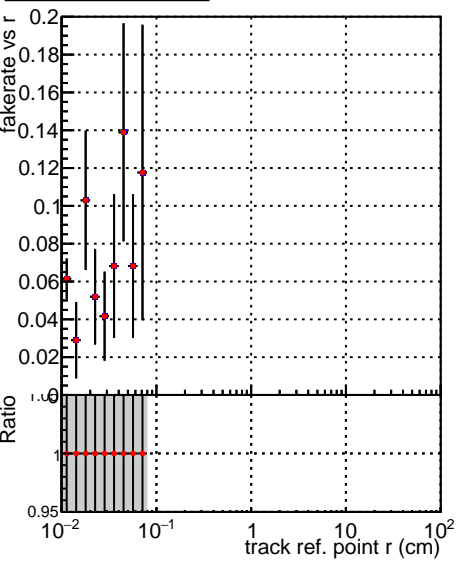
—●— DQM_V0001_R000000001_Global_mkFit_CANDFINAL100stable —●— DQM_V0001_R000000001_Global_mkFit_CANDFINAL100stable3
