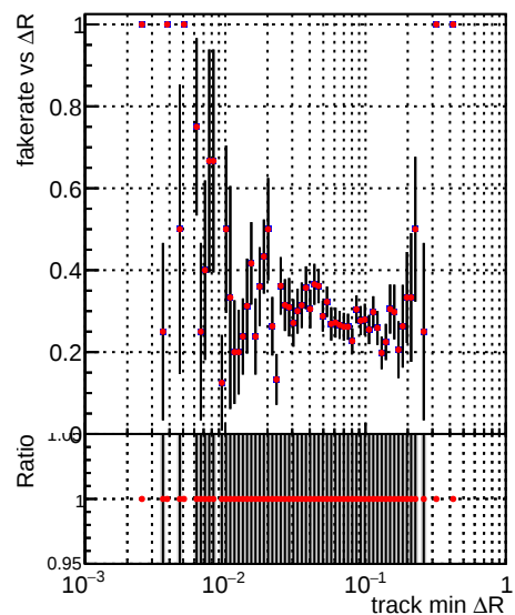
—●— DQM_V0001_R000000001_Global_mkFit_CANDFINAL100stable —●— DQM_V0001_R000000001_Global_mkFit_CANDFINAL100stable3
