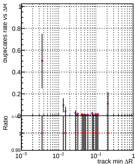
—●— DQM_V0001_R000000001_Global_mkFit_CANDFINAL100stable —●— DQM_V0001_R000000001_Global_mkFit_CANDFINAL100stable3
