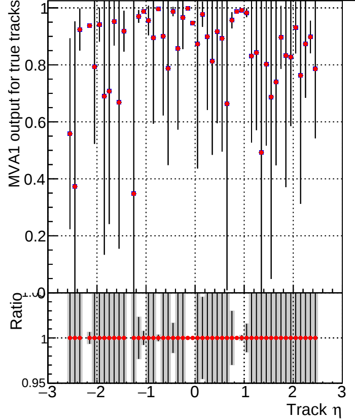
MVA1 of associated tracks (recoToSim) vs. track \eta Legend: ■ DQM_V0001_R000000001_Global_mkFit_CANDFINAL100stable ● DQM_V0001_R000000001_Global_mkFit_CANDFINAL100stable3
