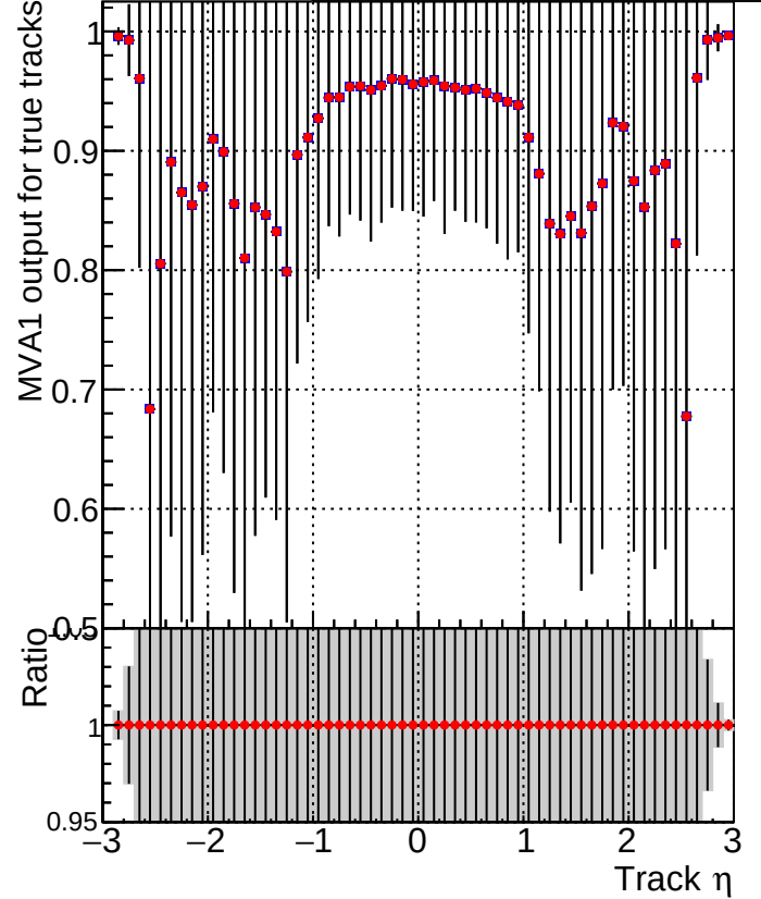
MVA1 of associated tracks (recoToSim) vs. track \eta ■ DQM_V0001_R000000001_Global_mkFit_CANDFINAL100stable ● DQM_V0001_R000000001_Global_mkFit_CANDFINAL100stable3
