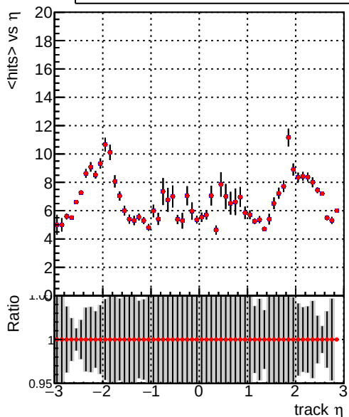
mean hit — DQM_V0001_R000000001_Global_mkFit_CANDFINAL100stable — DQM_V0001_R000000001_Global_mkFit_CANDFINAL100stable3
