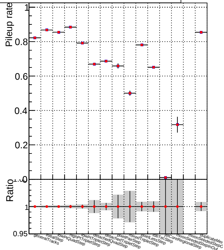
DQM_V0001_R000000001_Global_mkFit_CANDFINAL100stable3
