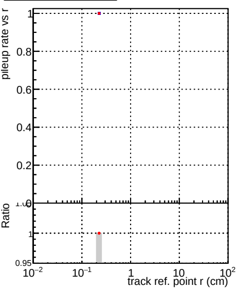
Legend: - Grey shaded region: DQM_V0001_R000000001_Global_mkFit_CANDFINAL100stable - Red dot with error bar: DQM_V0001_R000000001_Global_mkFit_CANDFINAL100stable3
