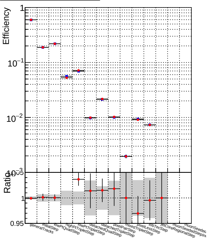
DQM_V0001_R000000001_Global_mkFit_1kstable DQM_V0001_R000000001_Global_mkFit_CAND1kstable
