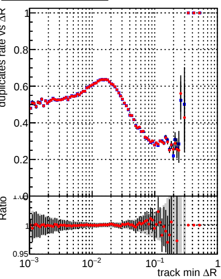
Legend: DQM_V0001_R000000001_Global_mkFit_1kstable (blue line with error bars), DQM_V0001_R000000001_Global_mkFit_CAND1kstable (red line with error bars)
