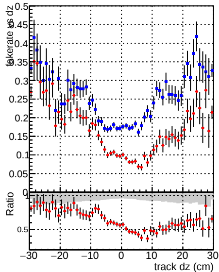
—■— DQM V0001_R000000001 Global mkFit 1kstable —●— DQM V0001_R000000001 Global mkFit CAND1kstable
