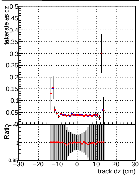
Fake rate vs dz —●— DQM_V0001_R0000000001 Global mkFit 1kstable —●— DQM_V0001_R0000000001 Global mkFit CAND1kstable
