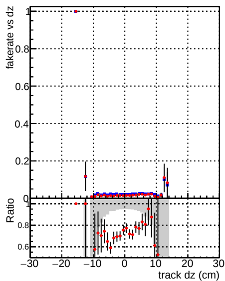
Fake rate vs dz —●— DQM_V0001_R0000000001_Global_mkFit_1kstable —●— DQM_V0001_R0000000001_Global_mkFit_CAND1kstable
