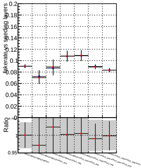
Fake rate vs. —●— DQM V0001_R000000001 Global mkFit 1kstable —●— DQM V0001_R000000001 Global mkFit CAND1kstable
