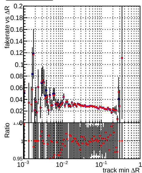
—●— DQM_V0001_R000000001_Global_mkFit_1kstable —●— DQM_V0001_R000000001_Global_mkFit_CAND1kstable
