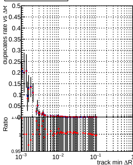
—●— DQM_V0001_R000000001_Global_mkFit_1kstable —●— DQM_V0001_R000000001_Global_mkFit_CAND1kstable
