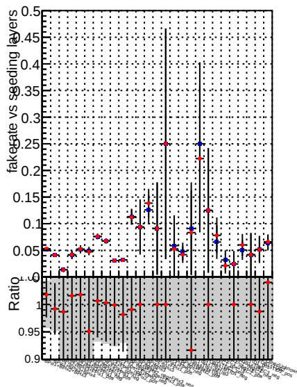
Fake rate vs. —●— DQM V0001_R000000001 Global mkFit 1kstable —●— DQM V0001_R000000001 Global mkFit CAND1kstable
