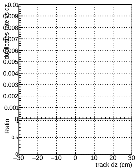
al__mkFit_1kstable al__mkFit_CAND1kstable
