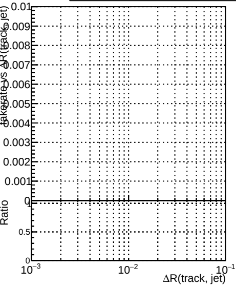
DQM_V0001_R000000001_Global_mkFit_1kstable DQM_V0001_R000000001_Global_mkFit_CAND1kstable
