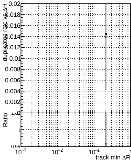
—●— DQM_V0001_R000000001_Global_mkFit_1kstable —●— DQM_V0001_R000000001_Global_mkFit_CAND1kstable
