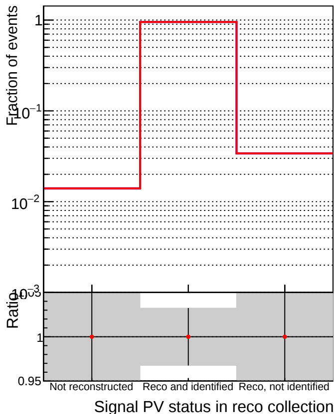
DQM_V0001_R000000001_Global_mkFit_1kstable DQM_V0001_R000000001_Global_mkFit_CAND1kstable
