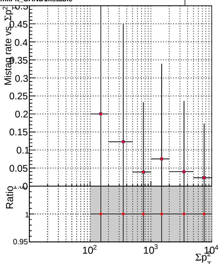
DQM_V0001_R000000001_Global_mkFit_1kstable DQM_V0001_R000000001_Global_mkFit_CAND1kstable
