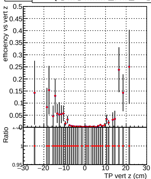
Efficiency vs vert z —●— DQM_V0001_R000000001_Global_mkFit_1kstable —●— DQM_V0001_R000000001_Global_mkFit_CAND1kstable
