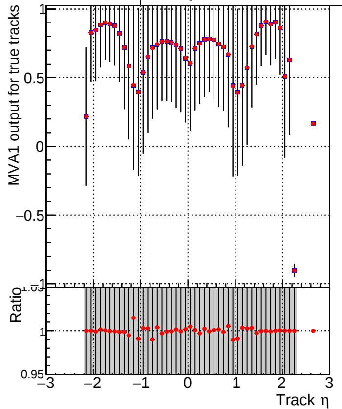
MVA1 of associated tracks (recoToSim) vs. track \eta Legend: ■ DQM_V0001_R000000001_Global_mkFit_1kstable ■ DQM_V0001_R000000001_Global_mkFit_CAND1kstable
