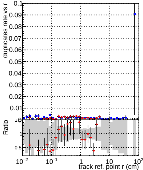
■ DQM_V0001_R000000001_Global_mkFit_1kstable ■ DQM_V0001_R000000001_Global_mkFit_CAND1kstable
