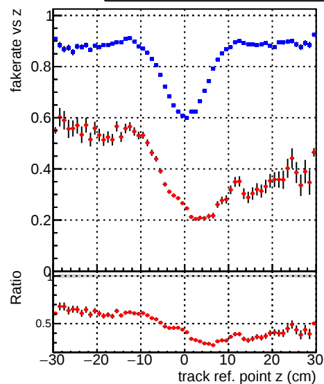
■ DQM_V0001_R000000001_Global_mkFit_1kstable ■ DQM_V0001_R000000001_Global_mkFit_CAND1kstable
