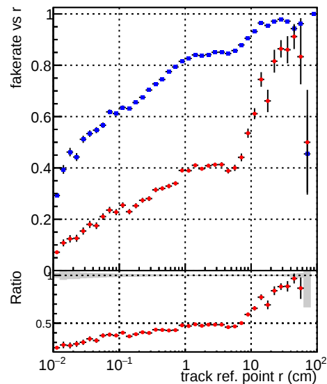
■ DQM_V0001_R000000001_Global_mkFit_1kstable ■ DQM_V0001_R000000001_Global_mkFit_CAND1kstable
