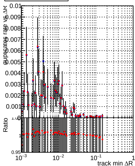
—●— DQM_V0001_R000000001_Global_mkFit_1kstable —●— DQM_V0001_R000000001_Global_mkFit_CAND1kstable
