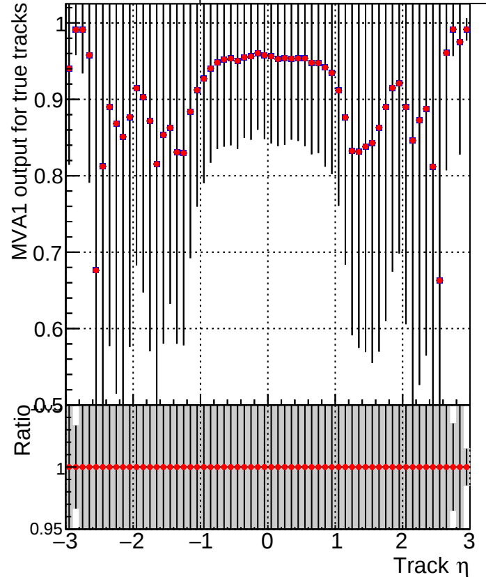
MVA1 of associated tracks (recoToSim) vs. track \eta Legend: ■ DQM_V0001_R000000001_Global_mkFit_1kstable ● DQM_V0001_R000000001_Global_mkFit_CAND1kstable
