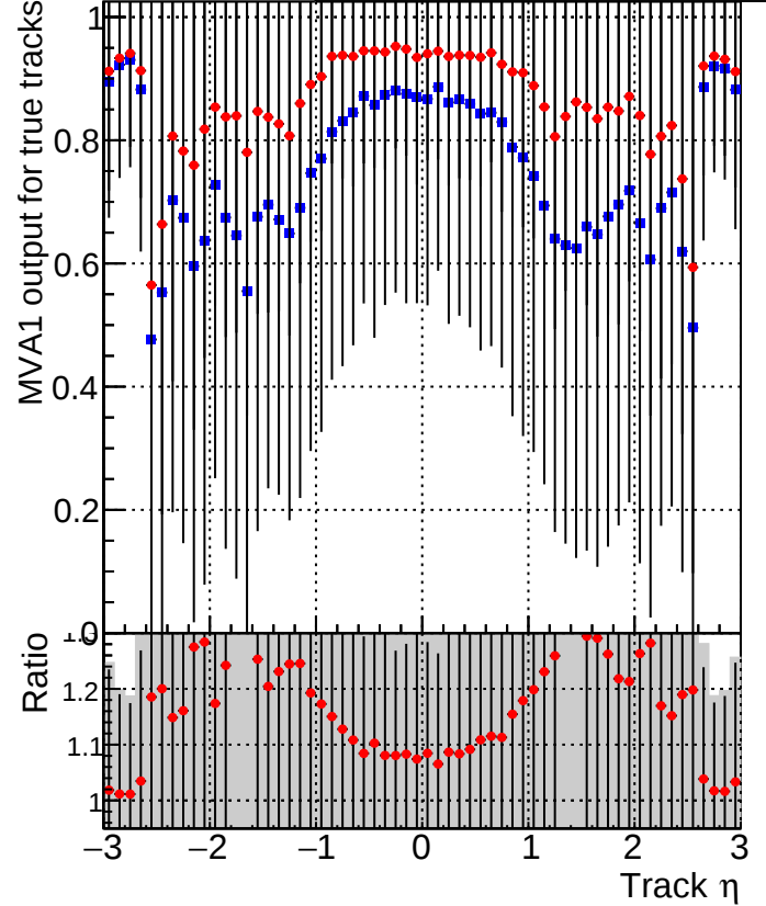
MVA1 of associated tracks (recoToSim) vs. track \eta Legend: Blue squares: DQM_V0001_R0000000001_Global_mkFit_1kstable Red diamonds: DQM_V0001_R0000000001_Global_mkFit_CAND1kstable
