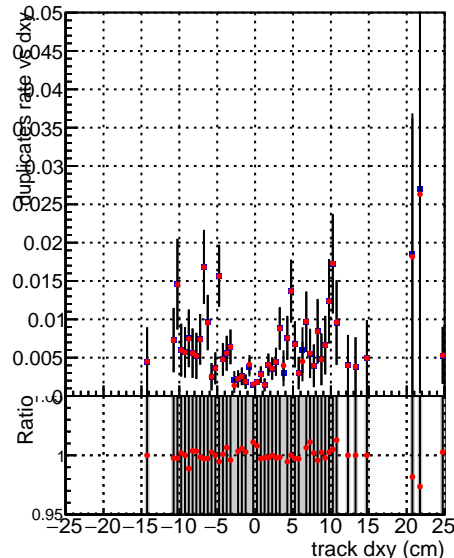
Duplicates Rate vs Dx
