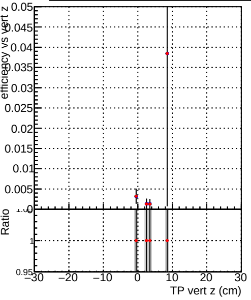
Efficiency vs. TP vert z (cm) Legend: DQM_V0001_R000000001_Global_mkFit_100stable DQM_V0001_R000000001_Global_mkFit_CAND100stable
