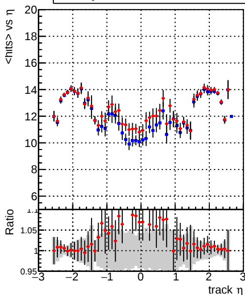
— DQM_V0001_R000000001_Global_mkFit_100stable — DQM_V0001_R000000001_Global_mkFit_CAND100stable
