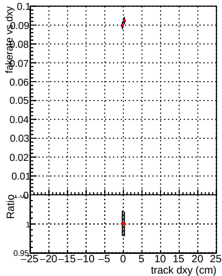
Fake rate vs d DQM V0001_R0000000001 Global mkFit 100stable DQM V0001_R0000000001 Global mkFit CAND100stable
