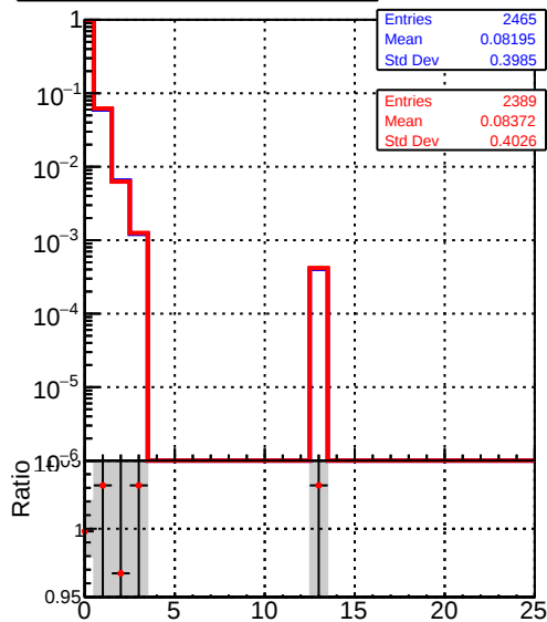
— DQM_V0001_R000000001_Global_mkFit_100stable — DQM_V0001_R000000001_Global_mkFit_CAND100stable
