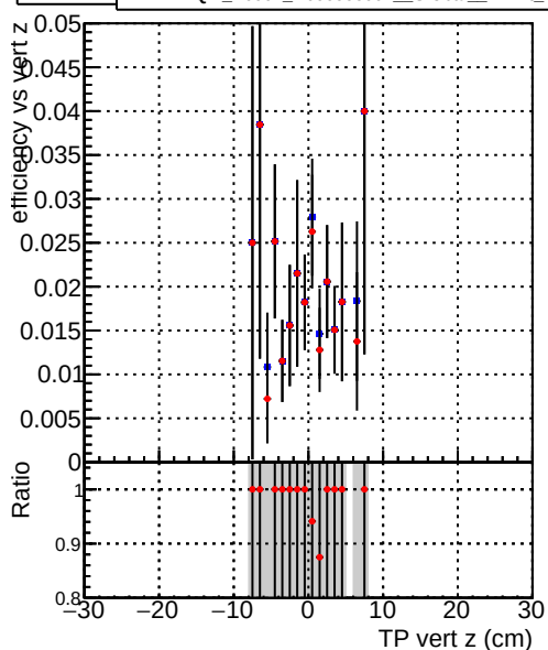
Efficiency vs. TP vert z (cm) — DQM_V0001_R000000001_Global_mkFit_100stable — DQM_V0001_R000000001_Global_mkFit_CAND100stable
