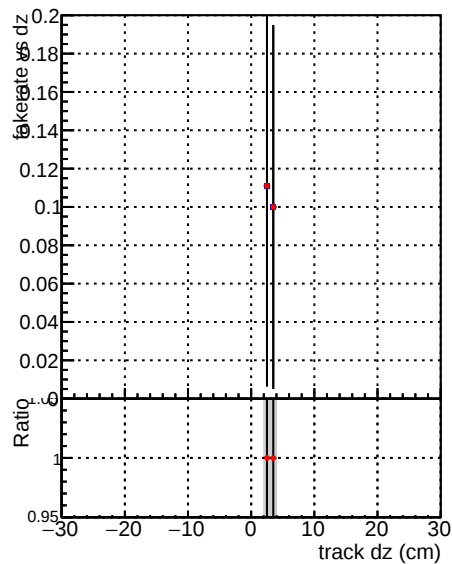
█ █ DQM_V0001_R000000001 Global mkFit_100stable █ █ DQM_V0001_R000000001 Global mkFit_CAND100stable
