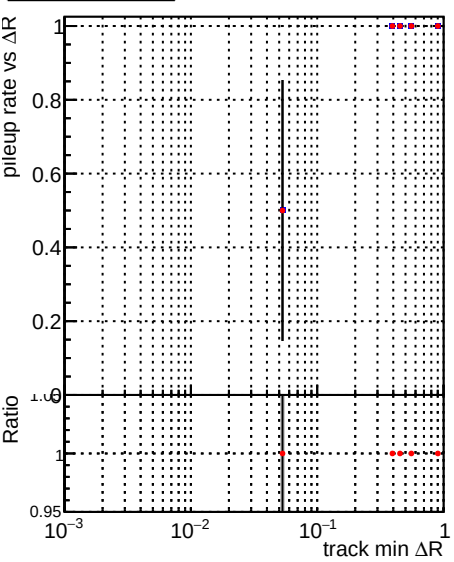
Legend: -█-█-█ DQM_V0001_R000000001_Global_mkFit_100stable -●-●-● DQM_V0001_R000000001_Global_mkFit_CAND100stable
