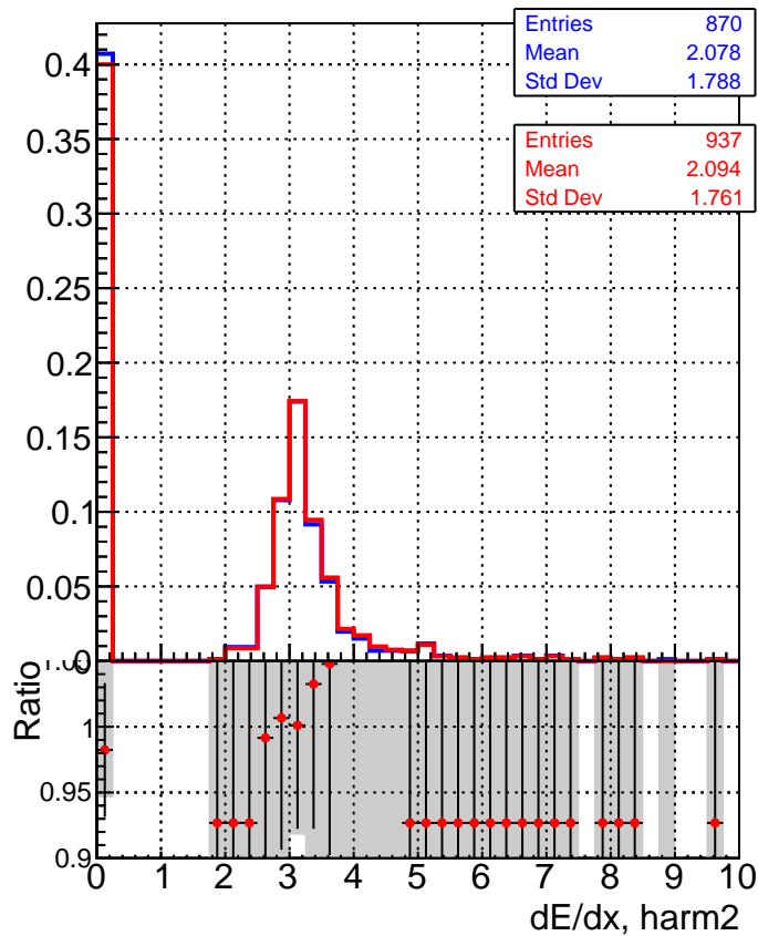
—■— DQM_V0001_R000000001_Global_mkFit_100stable —●— DQM_V0001_R000000001_Global_mkFit_CAND100stable
