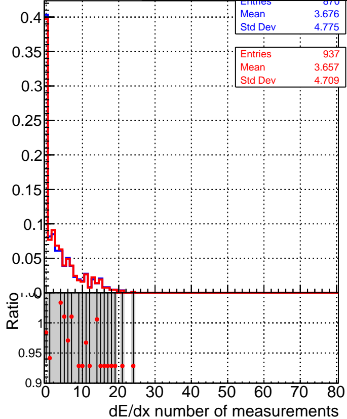
—■— DQM_V0001_R000000001_Global_mkFit_100stable —●— DQM_V0001_R000000001_Global_mkFit_CAND100stable
