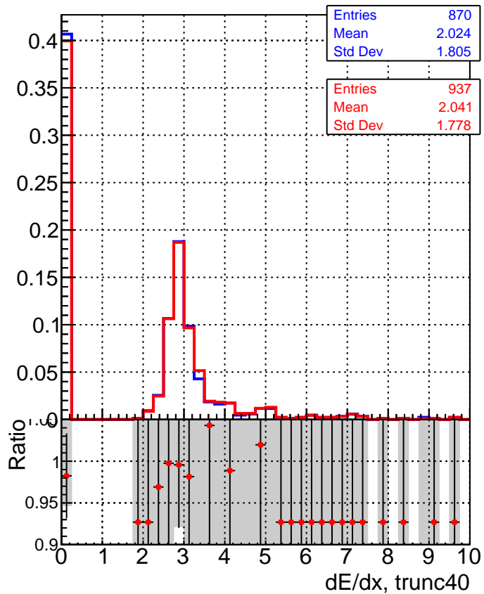
—■— DQM_V0001_R000000001_Global_mkFit_100stable —●— DQM_V0001_R000000001_Global_mkFit_CAND100stable
