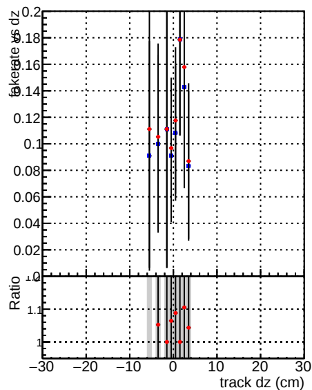
Fake rate vs dz —●— DQM_V0001_R0000000001_Global_mkFit_100stable —●— DQM_V0001_R0000000001_Global_mkFit_CAND100stable
