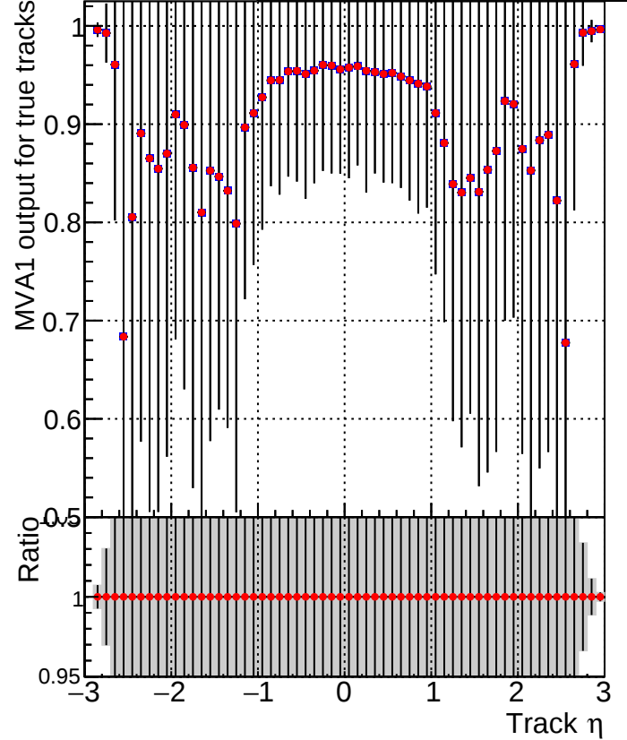
MVA1 of associated tracks (recoToSim) vs. track \eta ■ DQM_V0001_R000000001_Global_mkFit_100stable ● DQM_V0001_R000000001_Global_mkFit_CAND100stable
