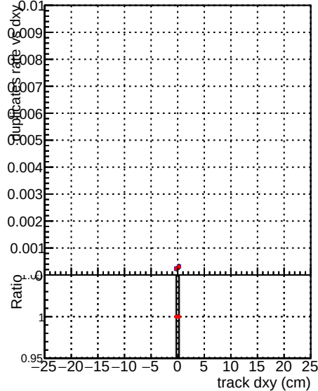
—●— DQM_V0001_R0000000001_Global_mkFit_100stable —●— DQM_V0001_R0000000001_Global_mkFit_CAND100stable
