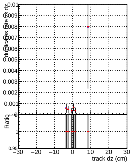
—●— DQM_V0001_R0000000001_Global_mkFit_100stable —●— DQM_V0001_R0000000001_Global_mkFit_CAND100stable
