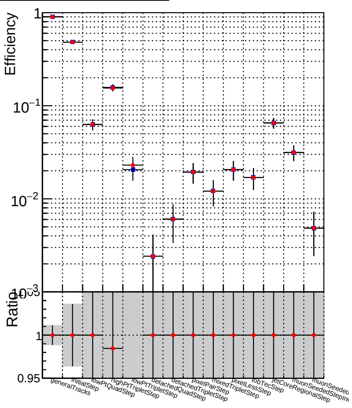
DQM_V0001_R000000001_Global_mkFit_100stable DQM_V0001_R000000001_Global_mkFit_CAND100stable
