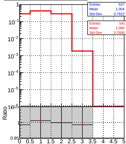
— DQM_V0001_R000000001_Global_mkFit_100stable — DQM_V0001_R000000001_Global_mkFit_CAND100stable
